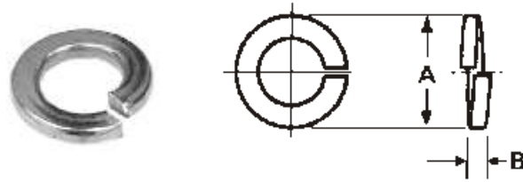
Stainless Steel Medium Split Washers
